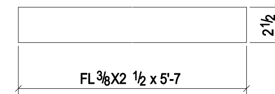
ONE - PLATE - p1531 (GR.-A36)
