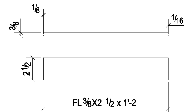
2 - PLATES - p1530 (GR.-A36)
