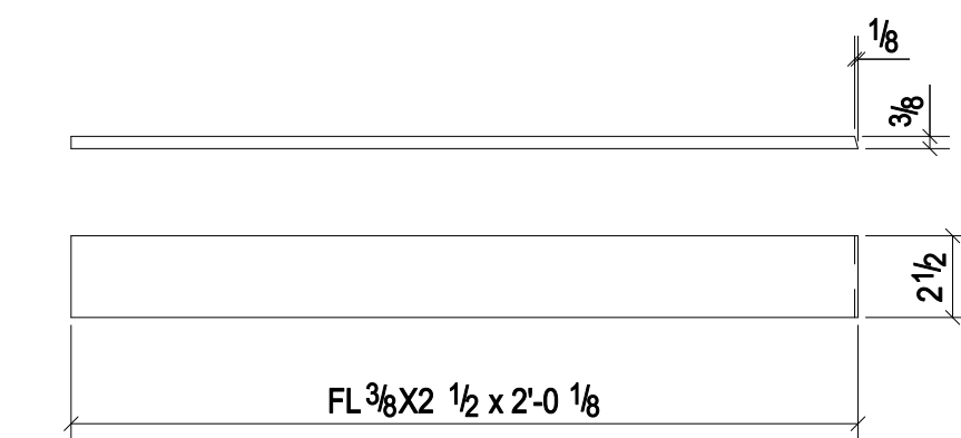
2 - PLATES - p1529 (GR.-A36)
